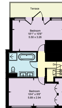
Fourth Floor
